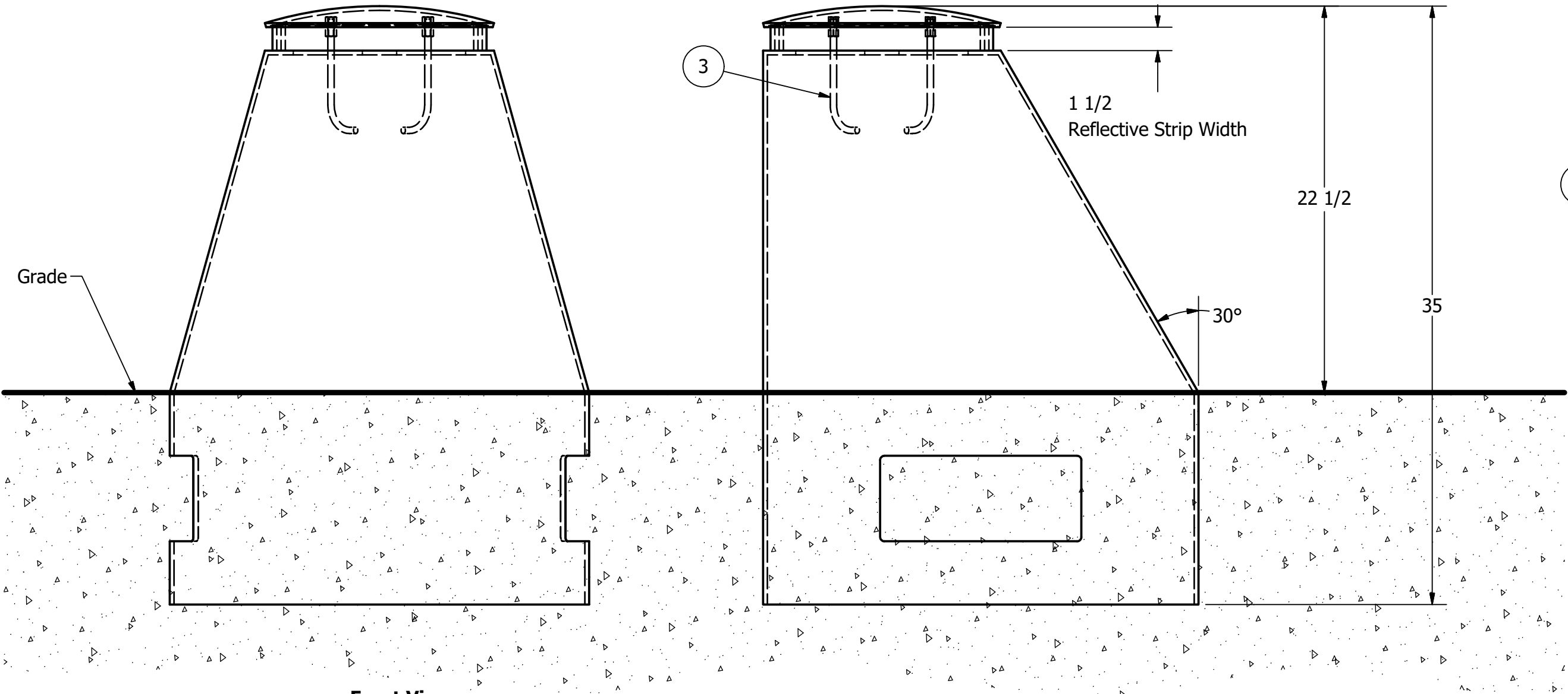
Side View
