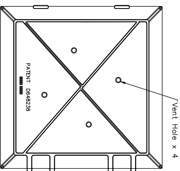
Underside View
