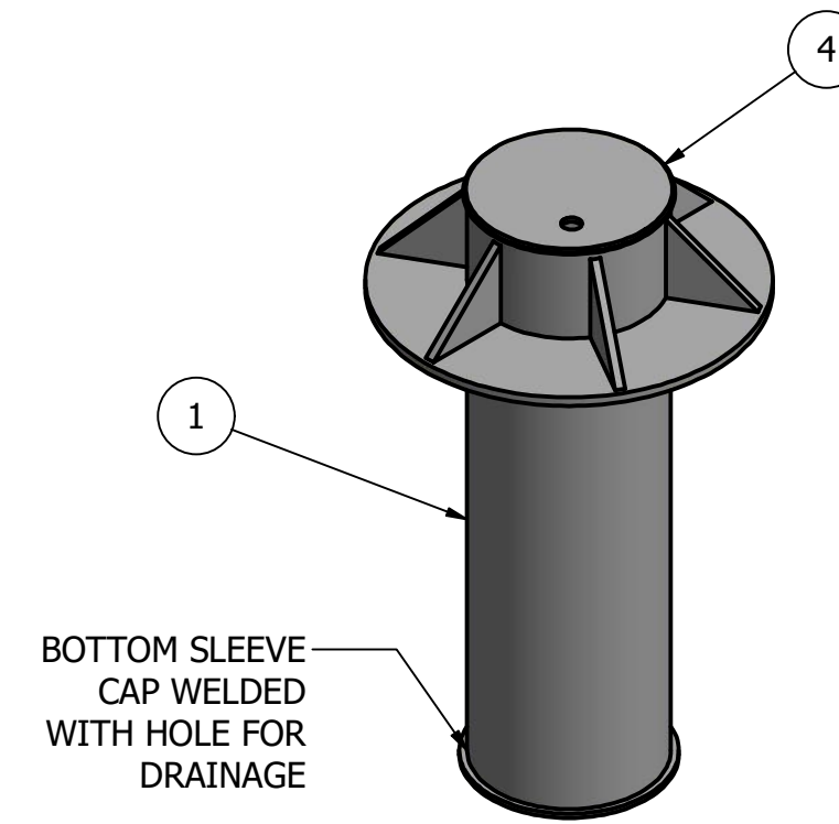
BOLLARD SLEEVE WITH CAP
