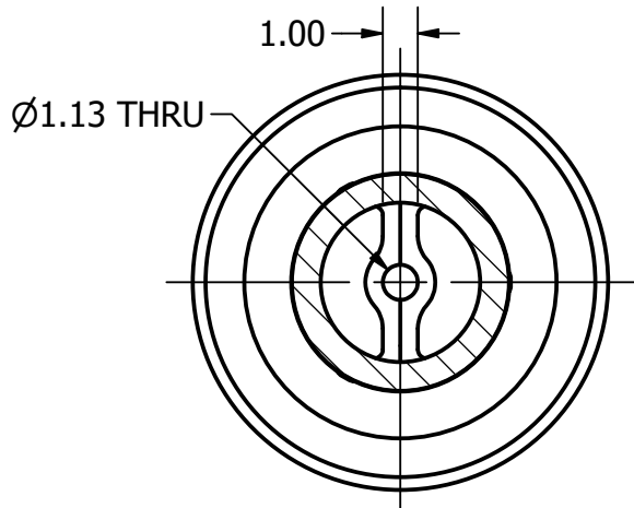
SECTION F-F SCALE 1 / 6
