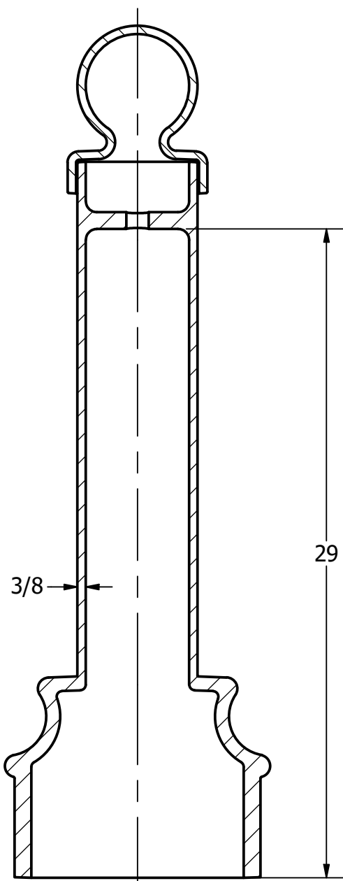
SECTION C-C SCALE 1 / 6
